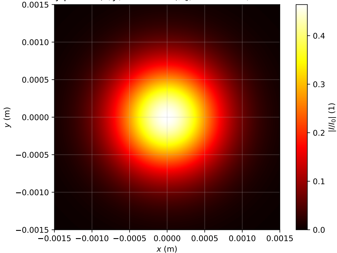
Intensity profile I(x, y, z = 3.105m)/I_0 , Pin=0.4Pcr, artificial time
